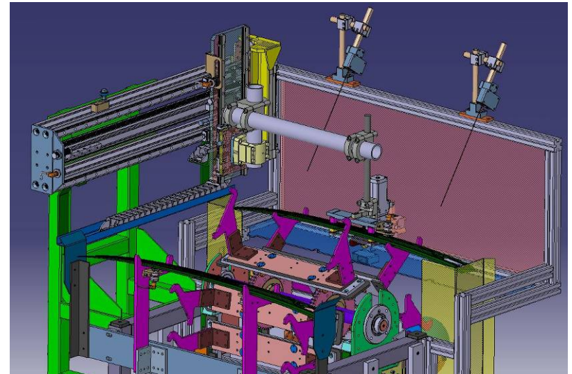
Detail: handling system for component unloading and transfer to robot
