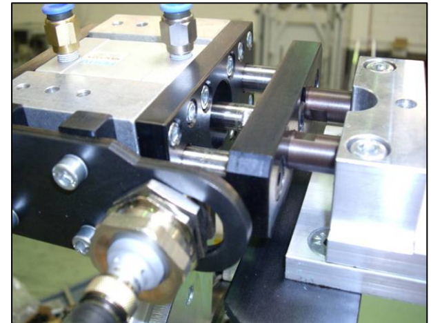
Fine positioning unit of transfer station for robotic unloading
