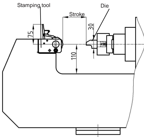
CBxx Series for Stamping
