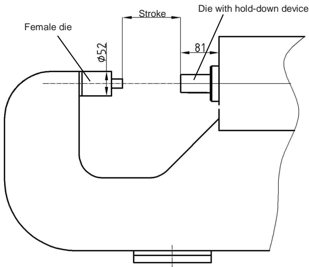
CBxx Series for Joining
