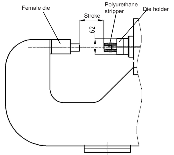
CBxx Series for Piercing
