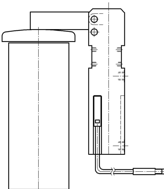
Application example No.2 Mini clamp applied as "lid-closing device"
