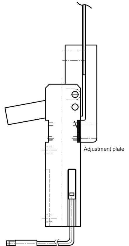
Application example No.3 Mini clamp applied for "locating of two sheets"
