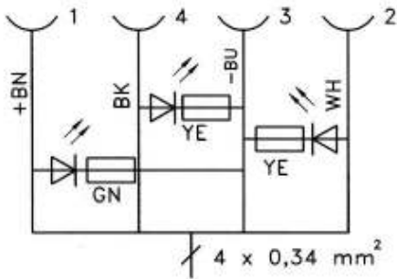
Pin assignment
